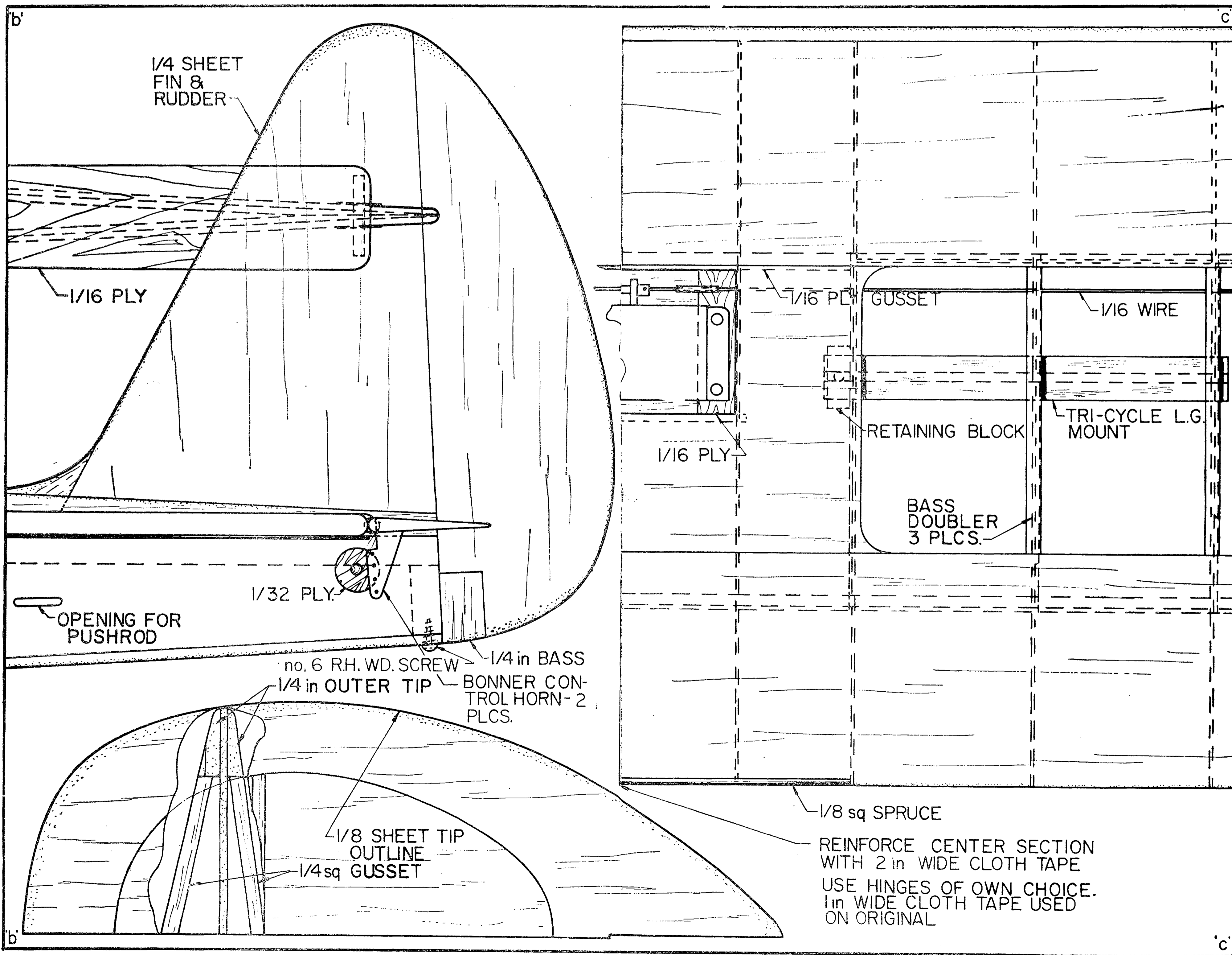
SECTION "A-A"
